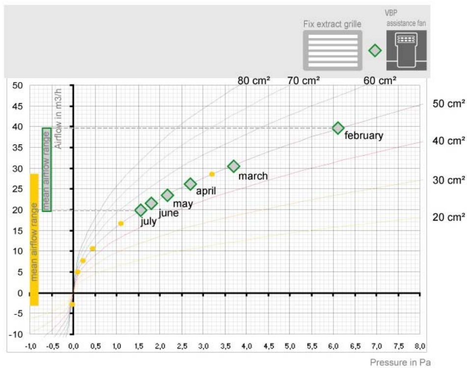
Figure 6 : Fix extract grille +assistance fan – Mean* monthly value of airflow / pressure
