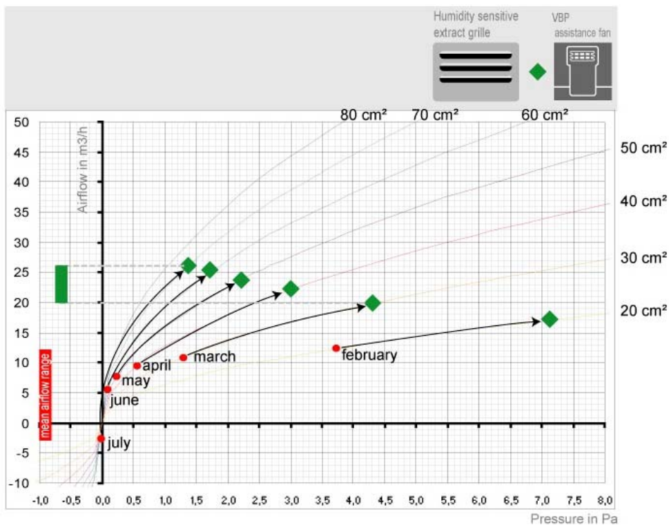
Figure 8 : Humidity sensitive extract grille + assistance fan – Mean* monthly value of airflow / pressure
