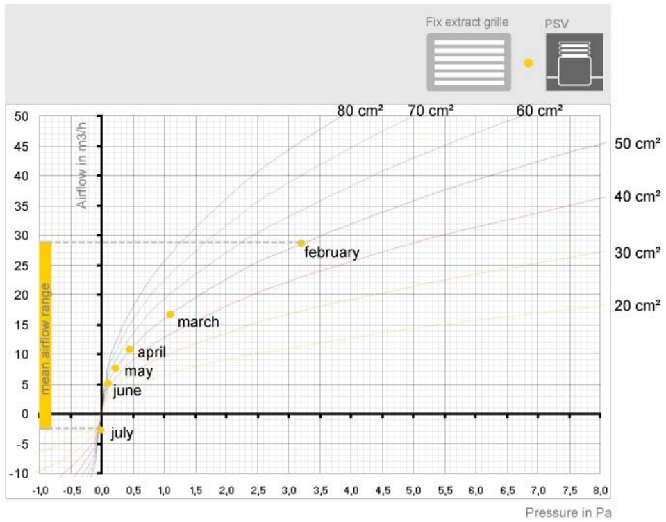
Figure 5 : Fix extract grille + PSV – Mean* monthly value of airflow / pressure
