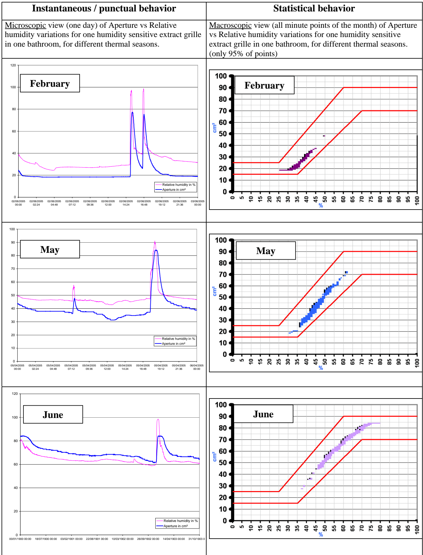
Figure 4 : Microscopic day-view and macroscopic monthly view of the variation of Aperture Vs Relative humidity of one humidity sensitive extract grille in one bathroom.
